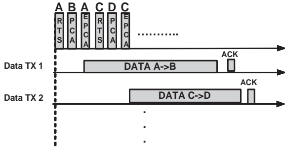
Fig. 9. RTS-PCA-EPCA-DATA-ACK packet exchange.
