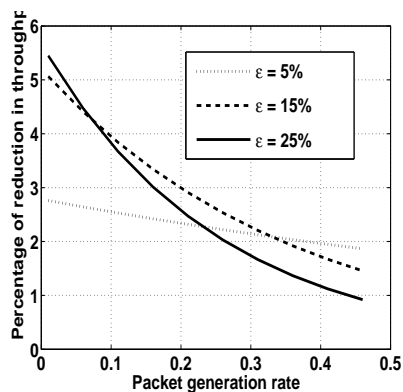
(b) Percentage of reduction in throughput vs. \lambda .
