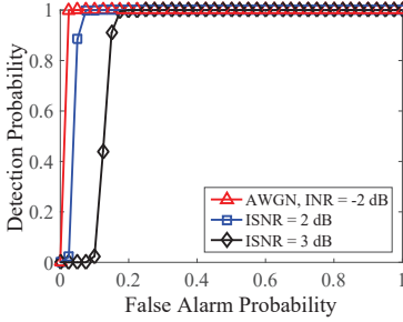
Fig. 11: ROC curves for various ISI levels (INR = -2 dB, STNR = 2 dB).
